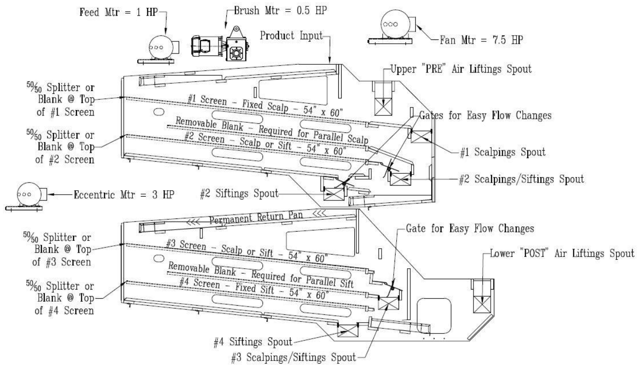
Q-SAGE 4x60-54-2+2-Brush Evolution Seed & Grain Cleaner Flow Diagram
